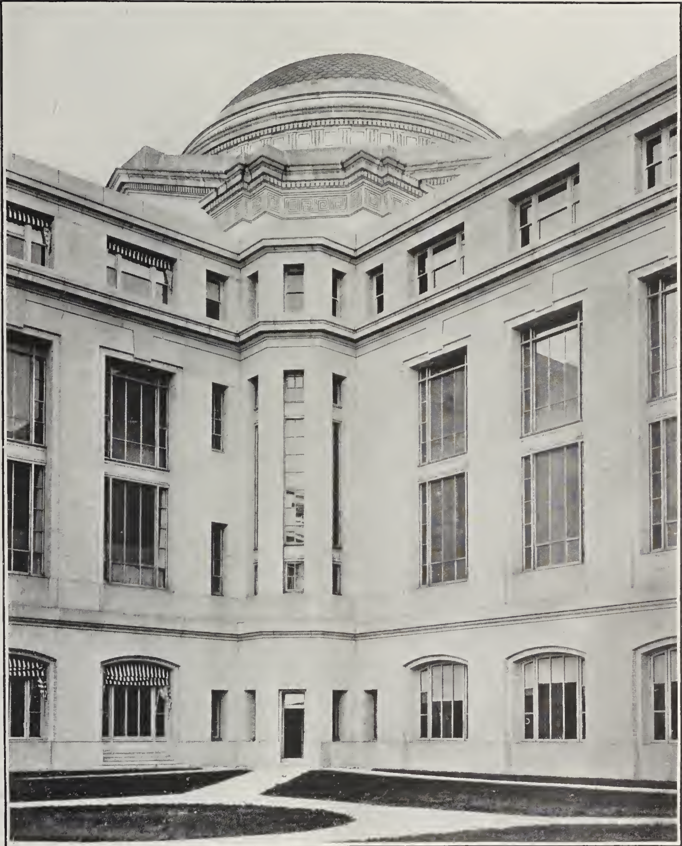
WEST COURT, LOOKING TOWARD THE SOUTH PAVILION AND ROTUNDA, AND SHOWING THE PROJECTION OF ONE OF THE STAIR TOWERS.
